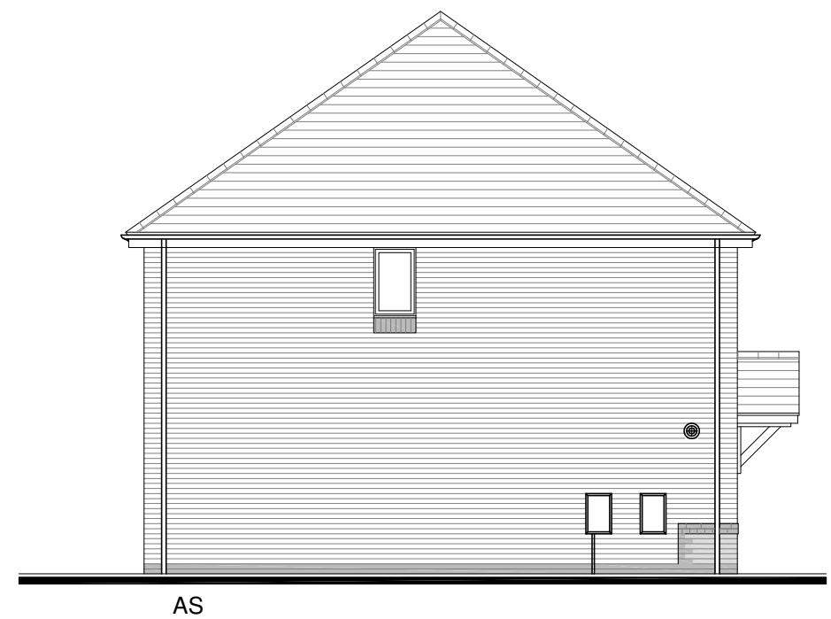
SIDE
