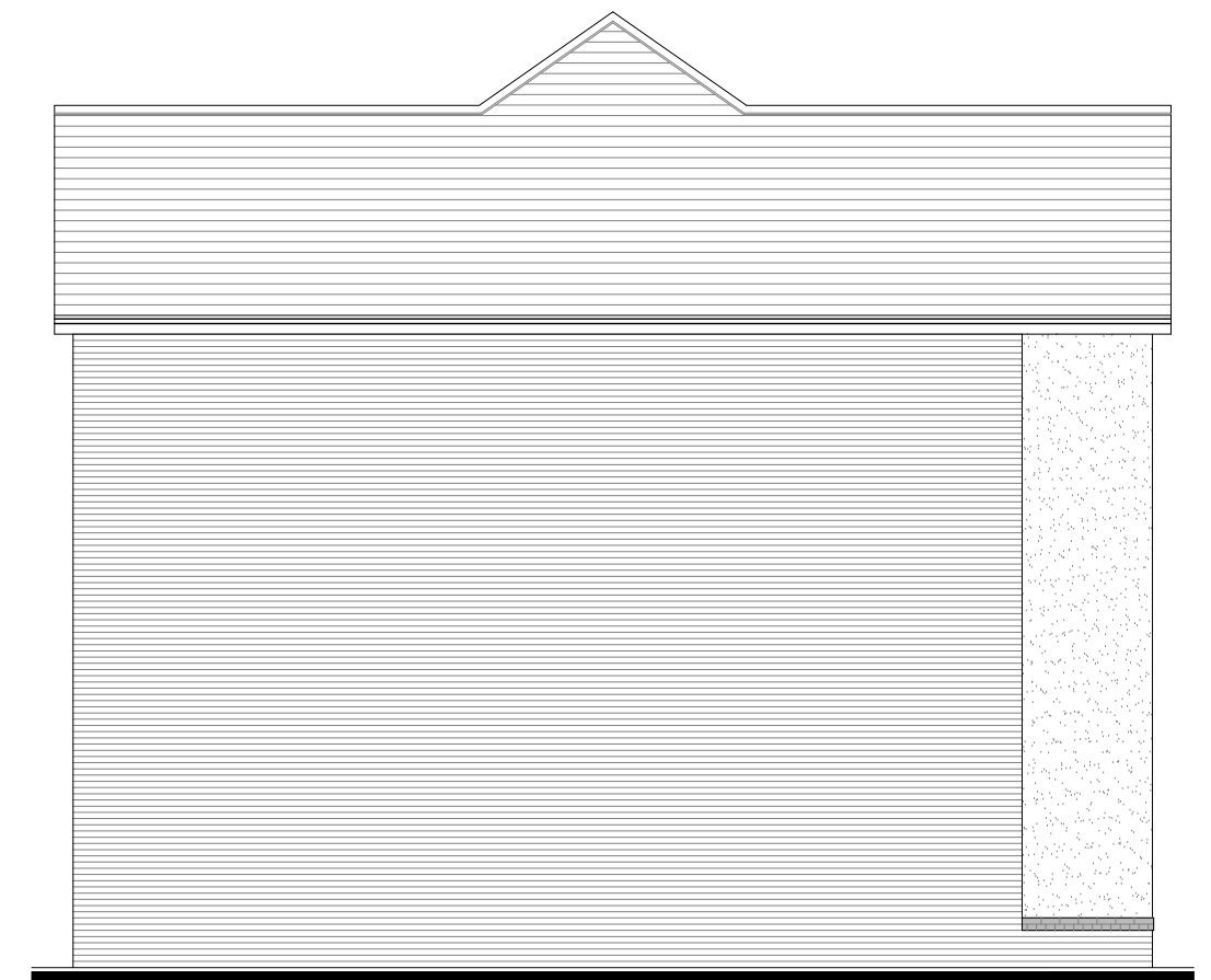
SIDE ELEVATION
