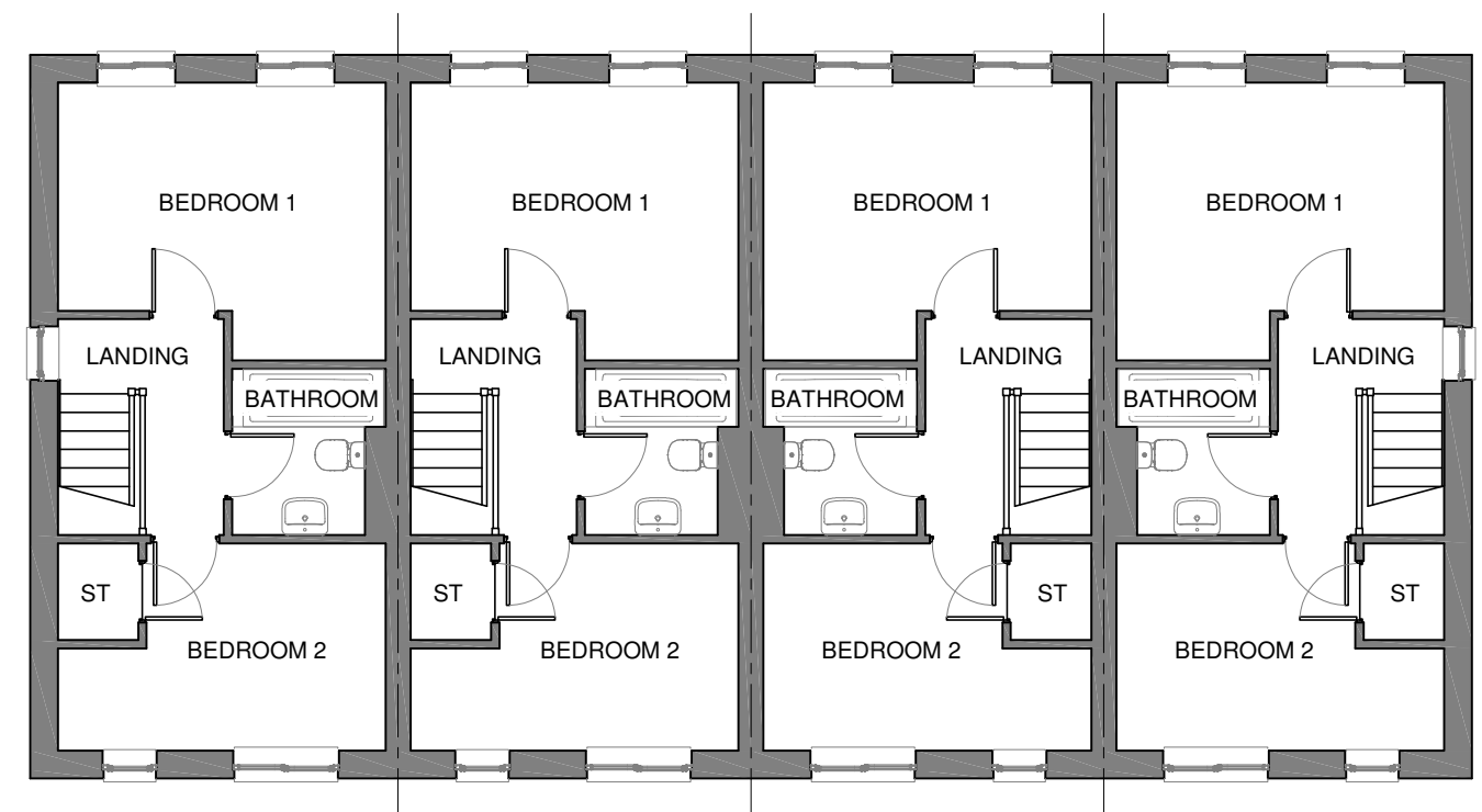
FIRST FLOOR
