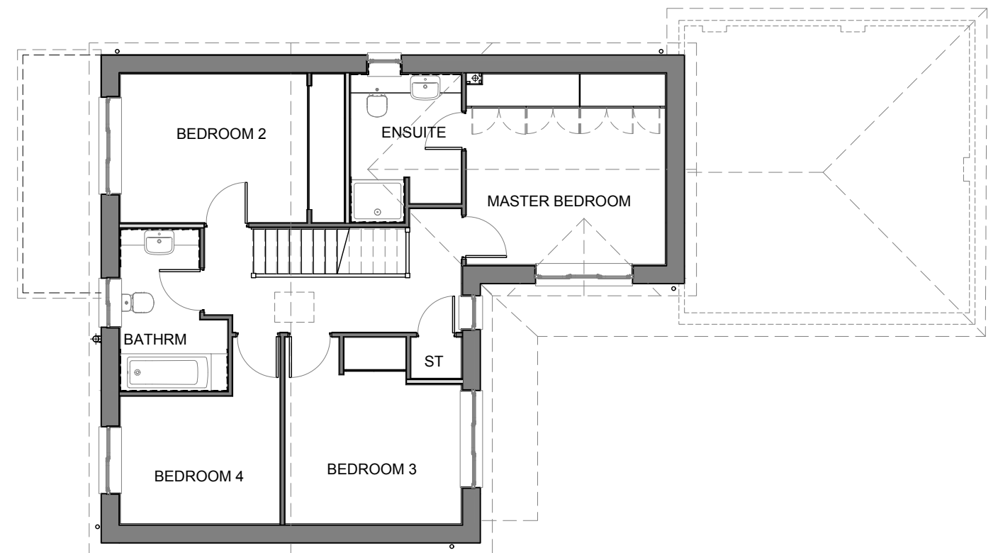
FIRST FLOORPLAN
