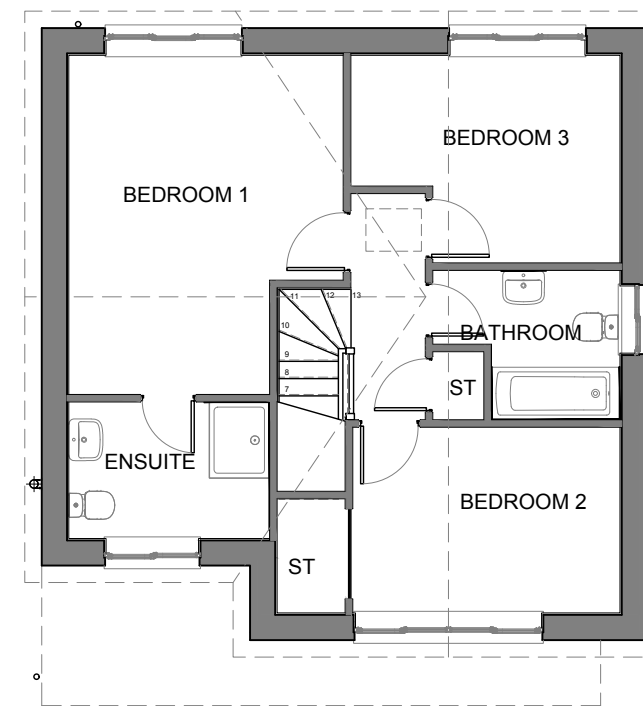
FIRST FLOORPLAN
