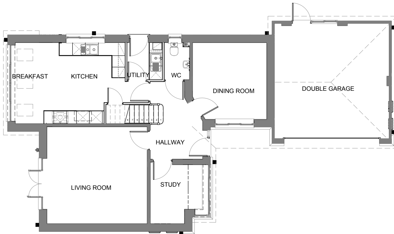
GROUND FLOORPLAN
