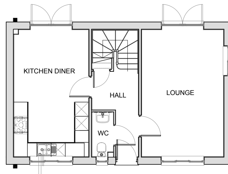
GROUND
