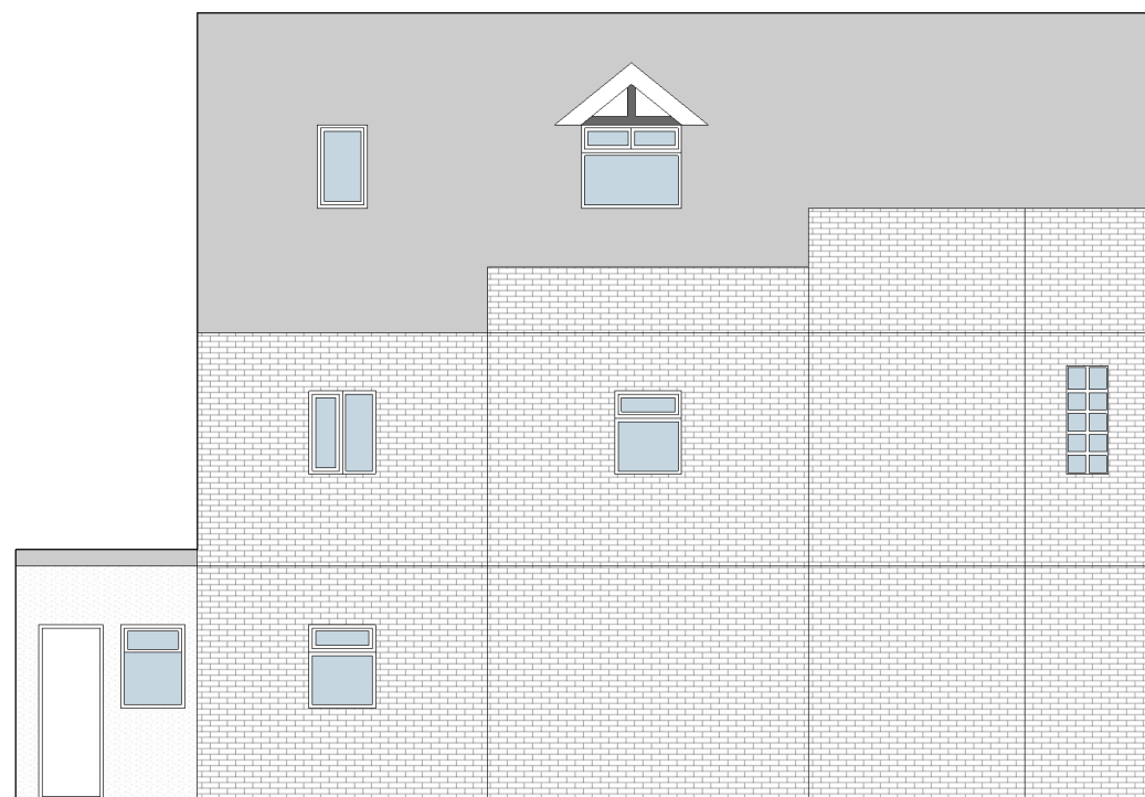
Elevation Borras Road
