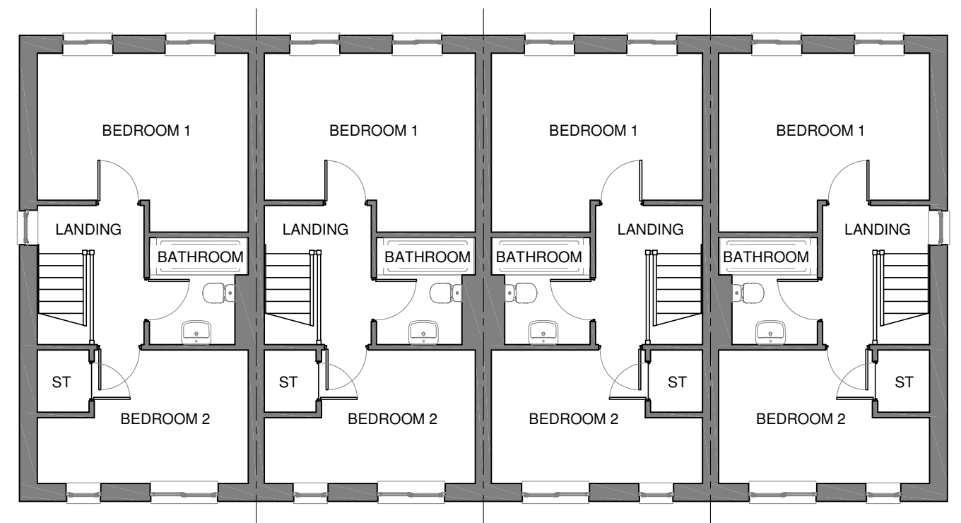
FIRST FLOOR
