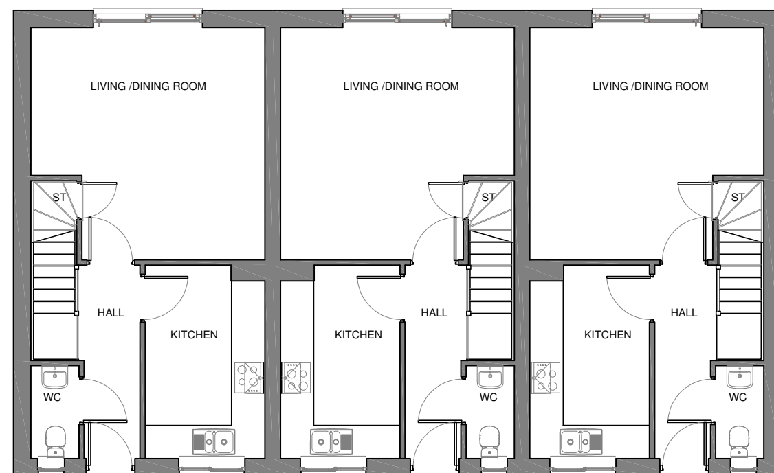
GROUND FLOOR
