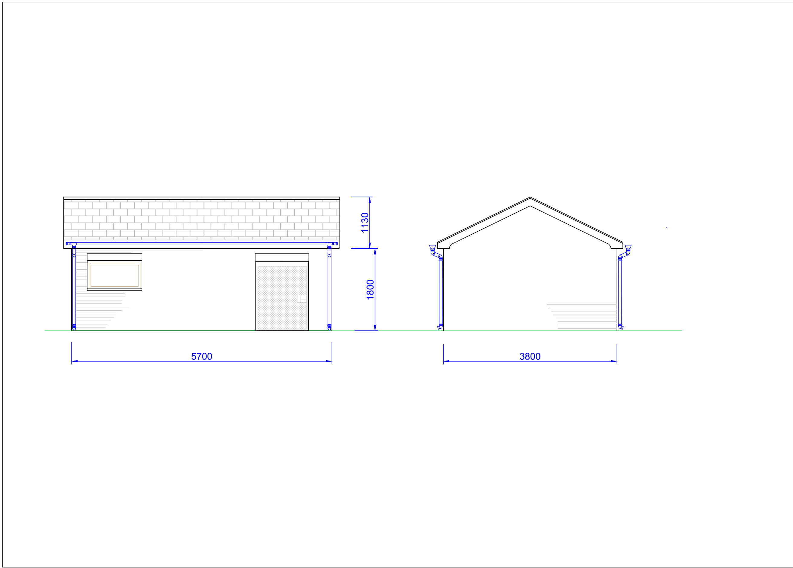
DISUED MICROTRAINER HOUSE (SCALE 1:50)
