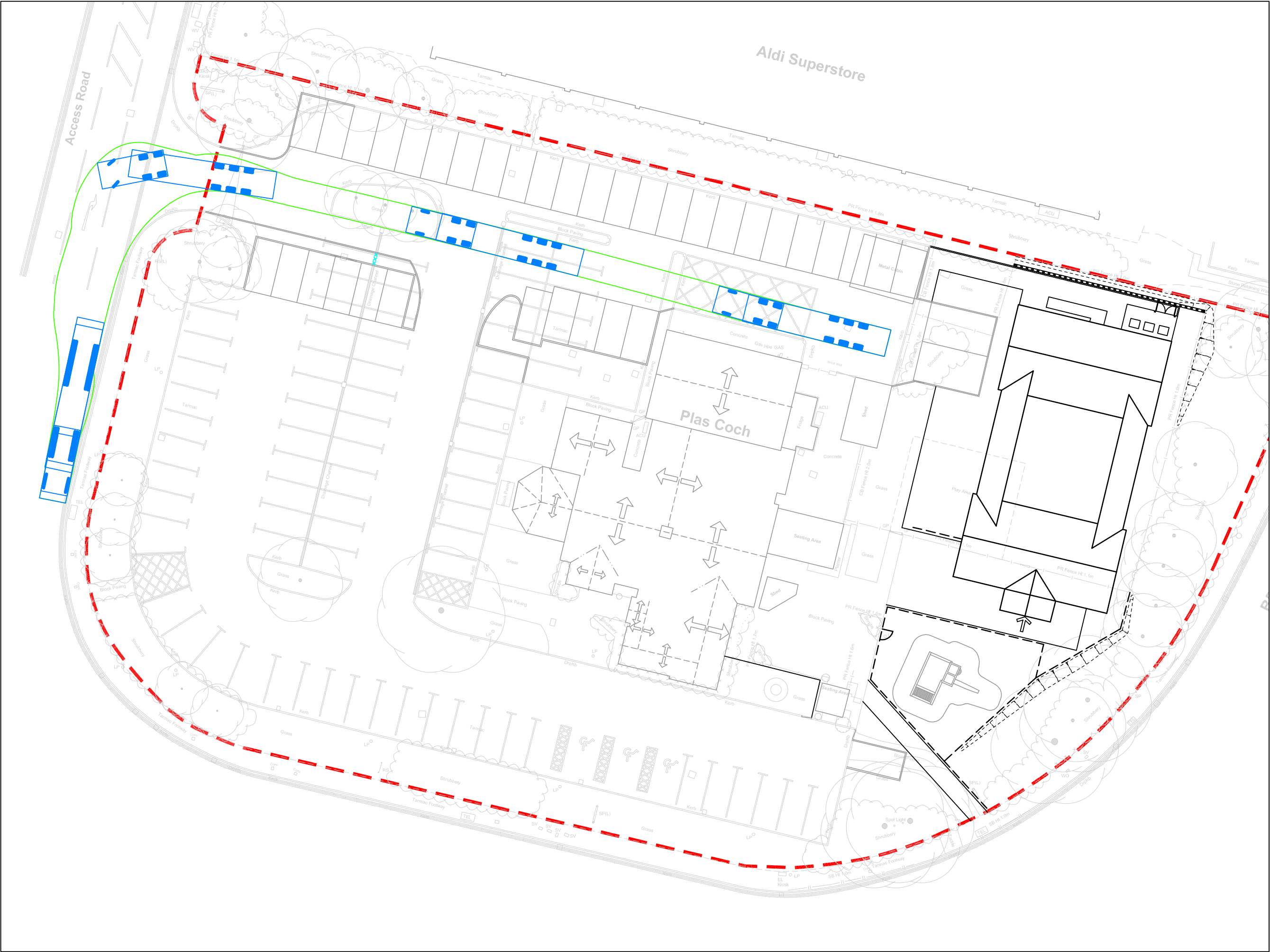
16.5m MAXIMUM LEGAL ARTICULATED VEHICLE – OUT
