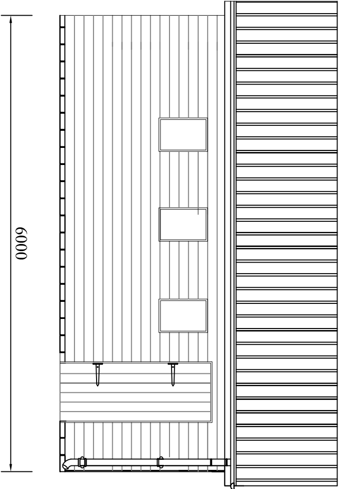
South Elevation
