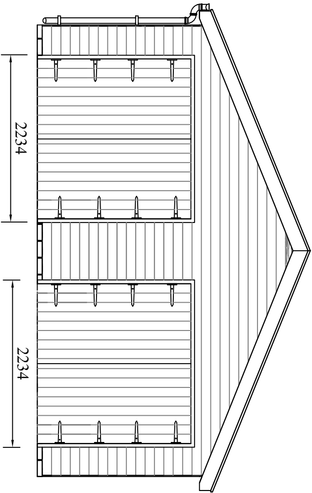
West Elevation
