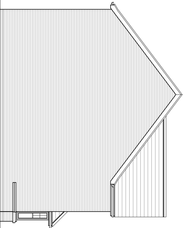
SIDE ELEVATION
