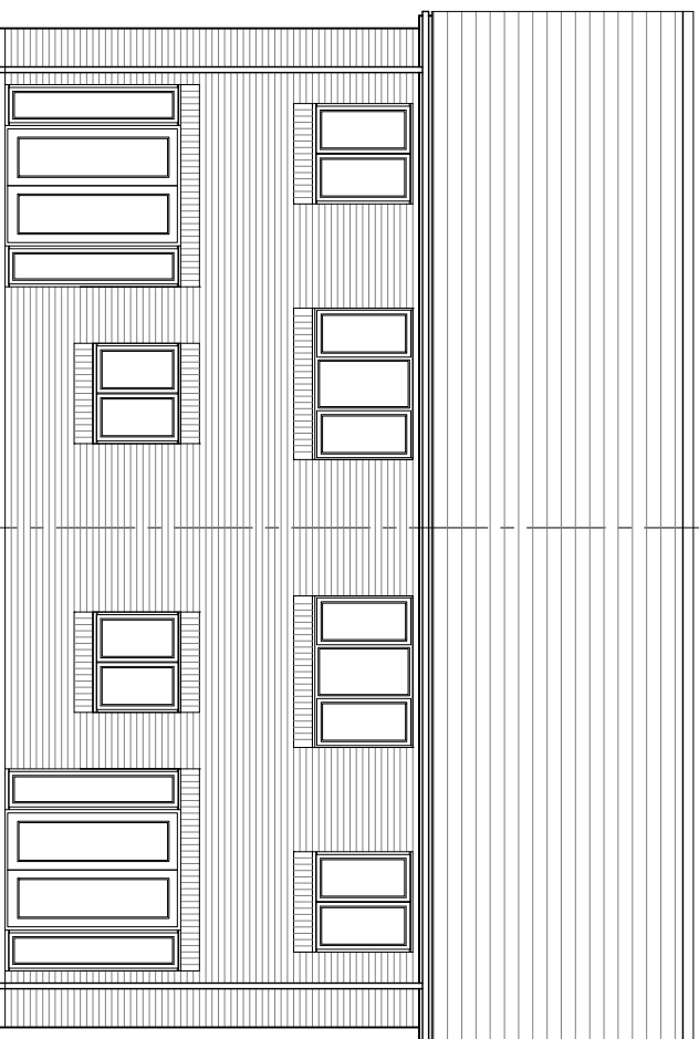
REAR ELEVATION
