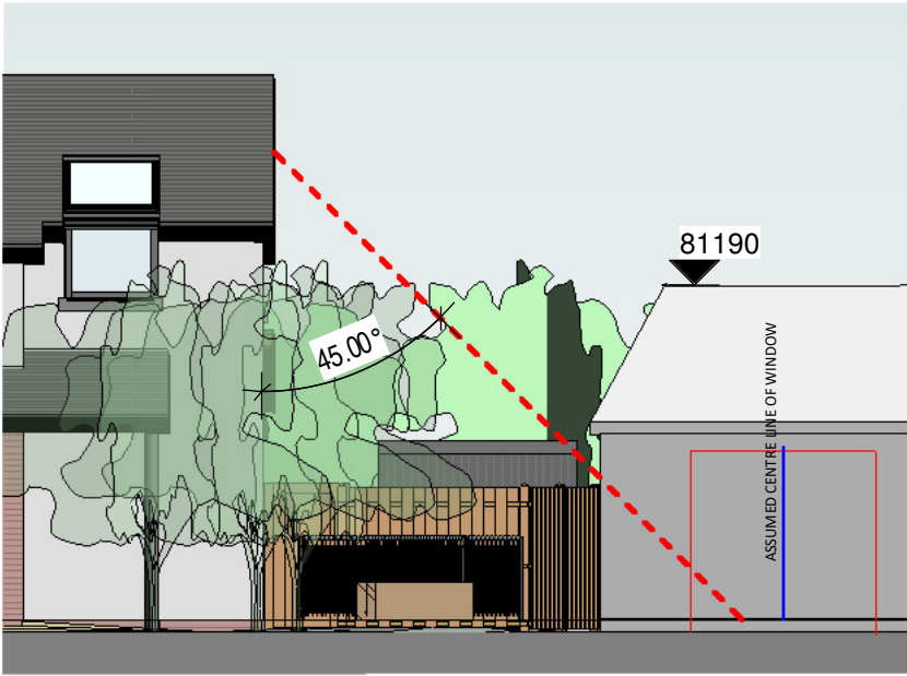
45 DEGREE RULE - ELEVATION
