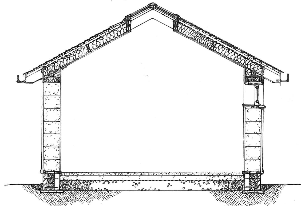
Construction Section
