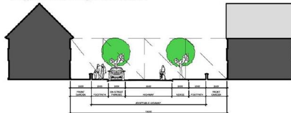
3. Typical Street - Height : Width ratio 1:3.5
