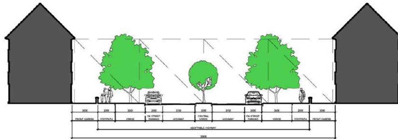
1. Typical Boulevard - Height : Width ratio 1:4
