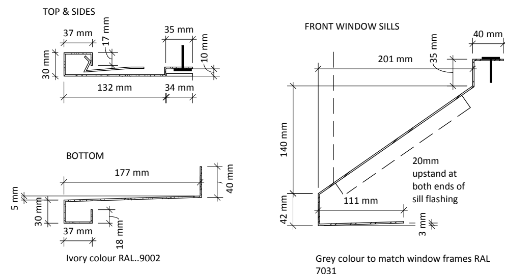
Window Surround profiles FF & SF front windows 1 : 5
