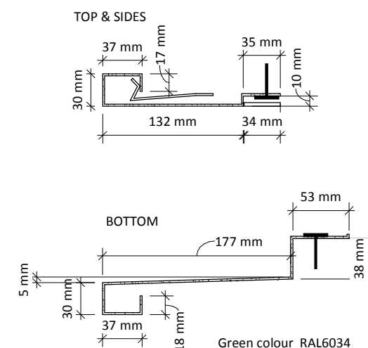
Window Surround profiles Side and rear windows 1 : 5
