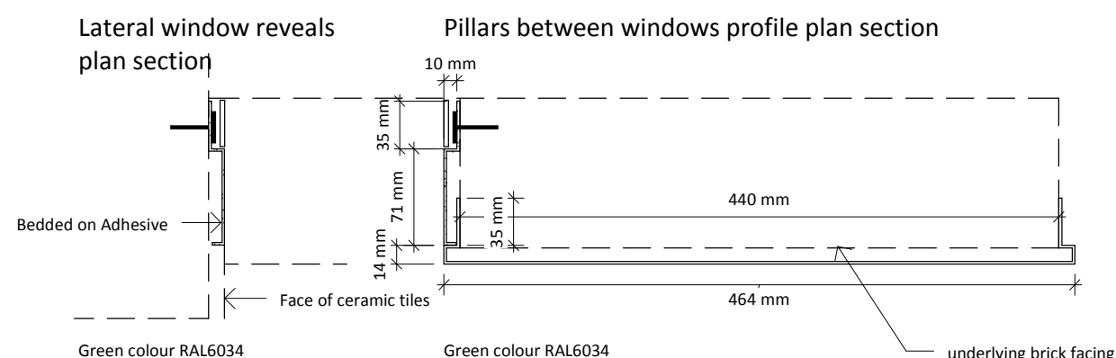
Window Surround profiles GF Shopfront 1 : 5
