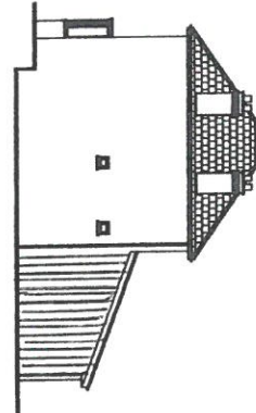
EXISTING SIDE ELEVATION
