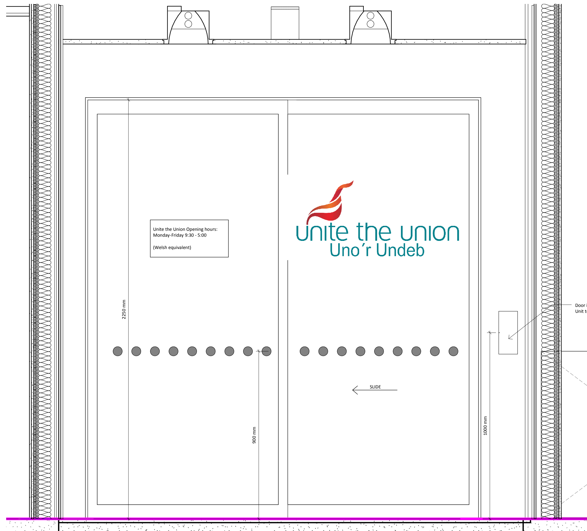
3 Main Door Entrance - Elevation 1 : 10
