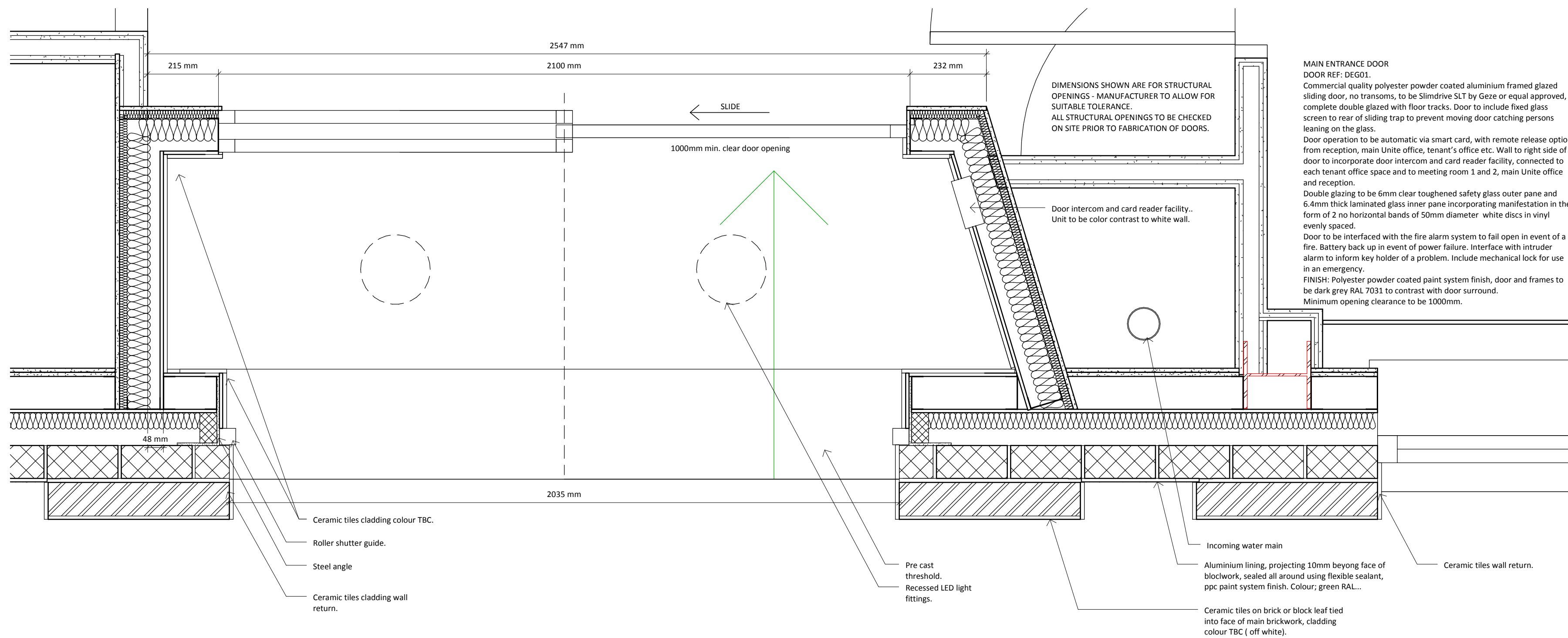
1 Porch Main Entrance - Detail Plan 1 : 10
