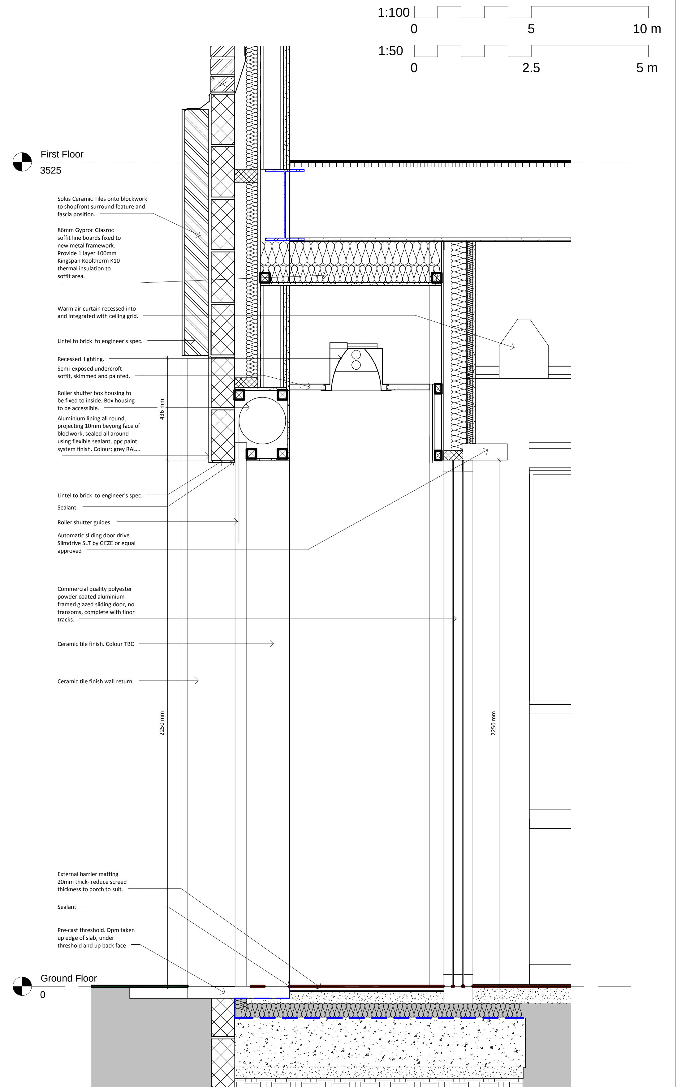
2 Porch Main Entrance - Detail Section 1 : 10
