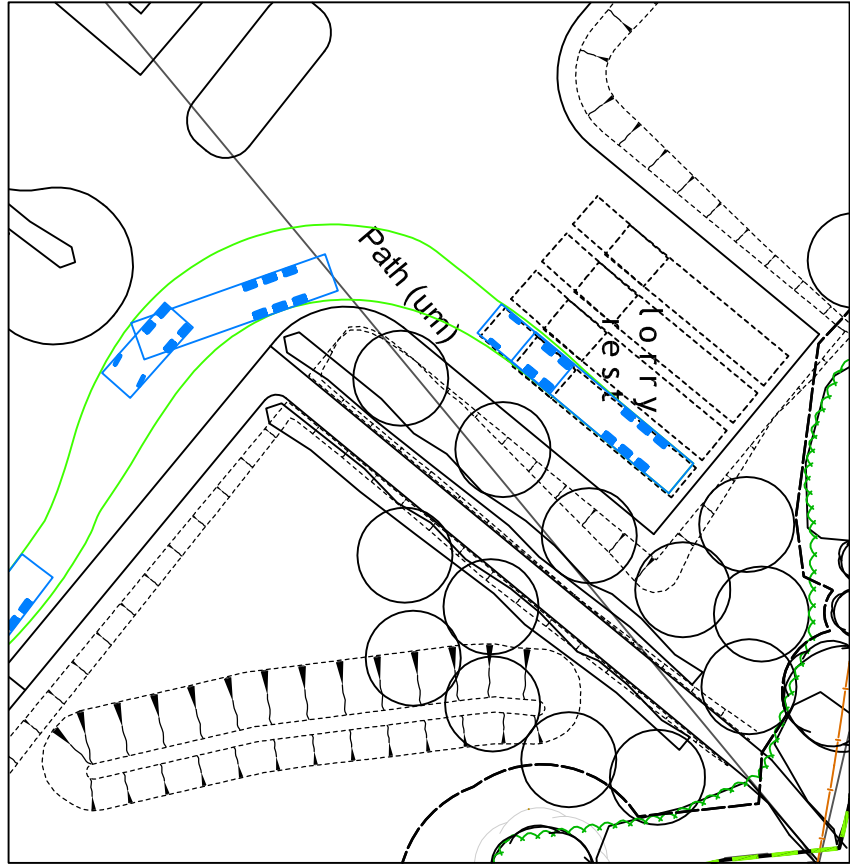
16.5m MAXIMUM LEGAL ARTICULATED VEHICLE – OUT (LORRY REST 1)
