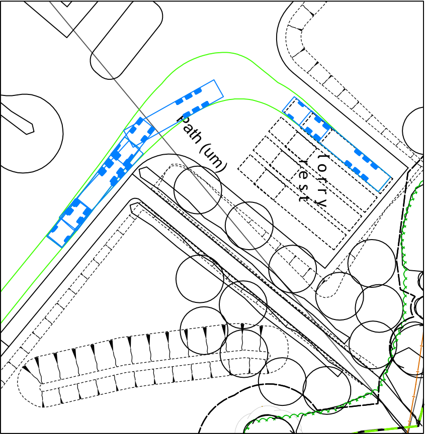
16.5m MAXIMUM LEGAL ARTICULATED VEHICLE – IN (DELIVERY BAY)
