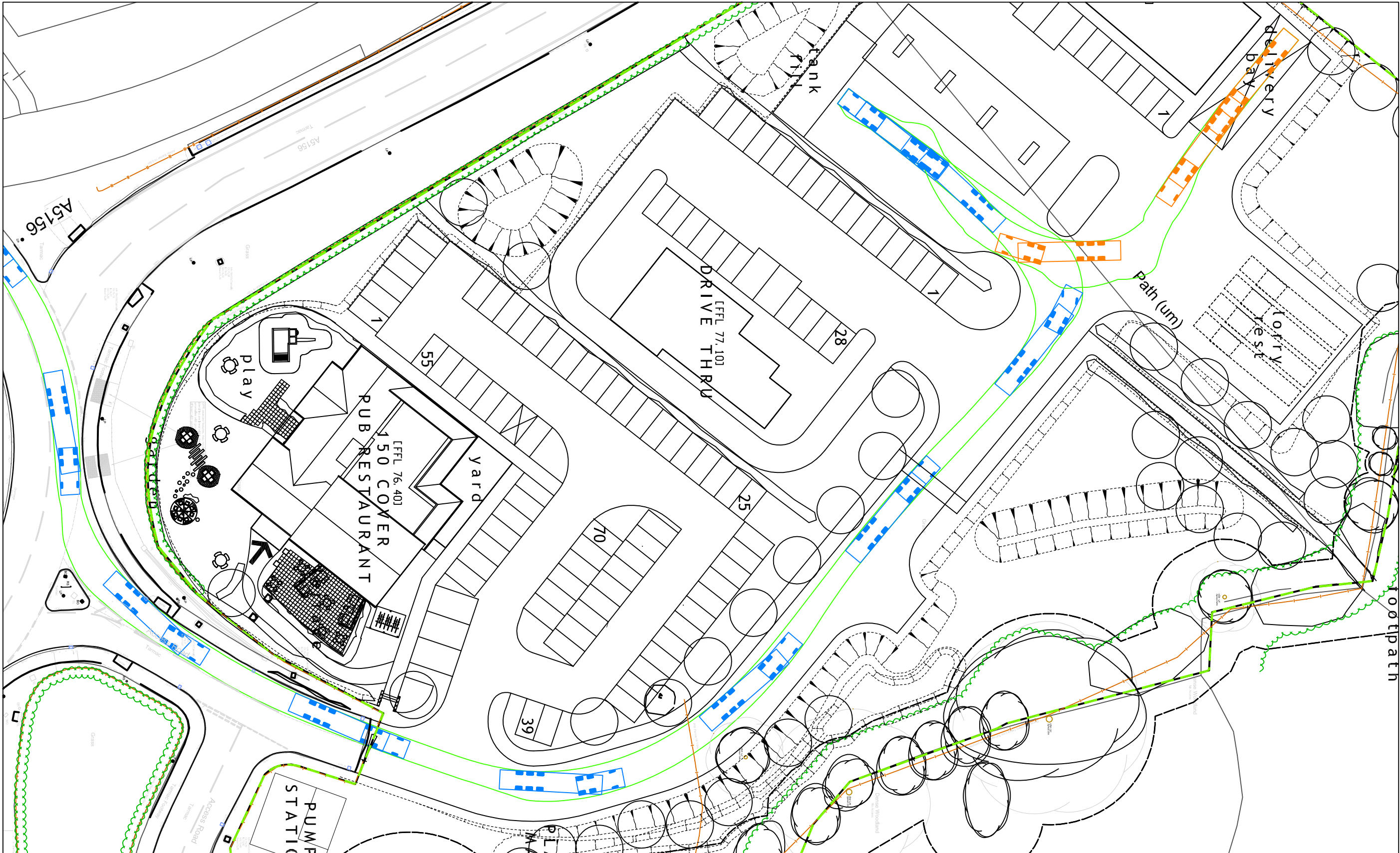
16.5m MAXIMUM LEGAL ARTICULATED VEHICLE – IN (DELIVERY BAY)
