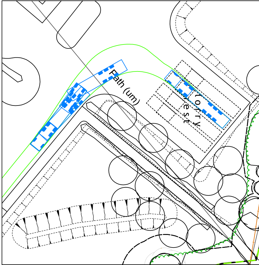
16.5m MAXIMUM LEGAL ARTICULATED VEHICLE – OUT (LORRY REST 3)
