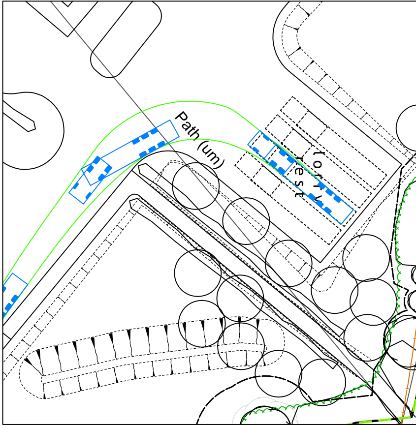
16.5m MAXIMUM LEGAL ARTICULATED VEHICLE – OUT (LORRY REST 2)
