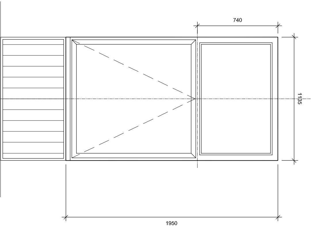
Typical Cedar Feature Elevation - 1:20
