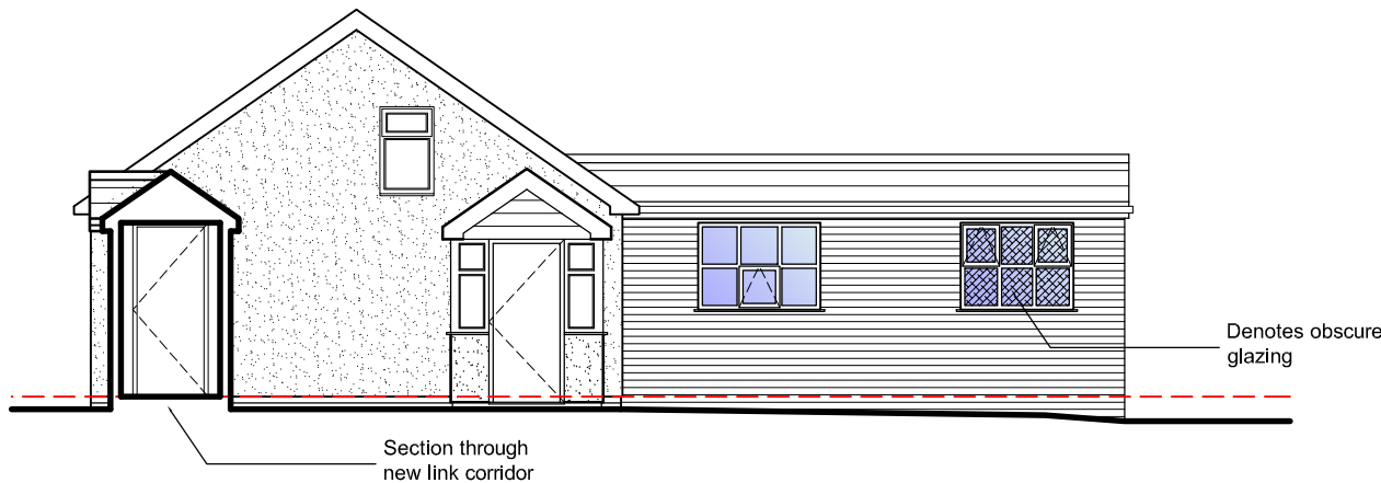
SIDE ELEVATION
