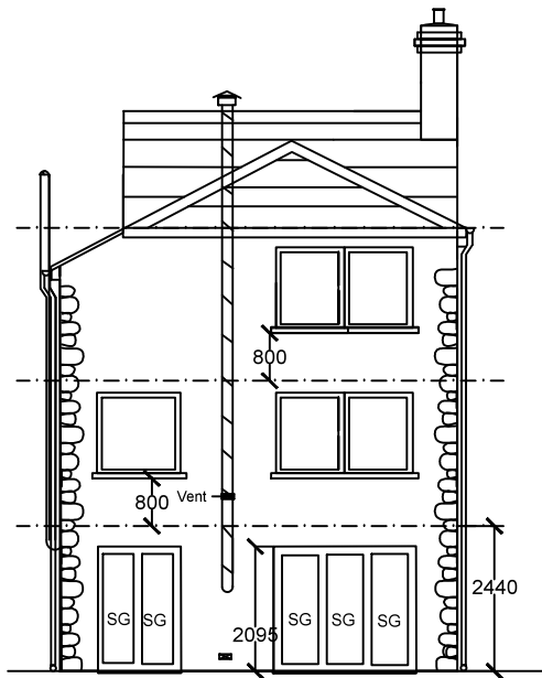
ELAVATION 3
