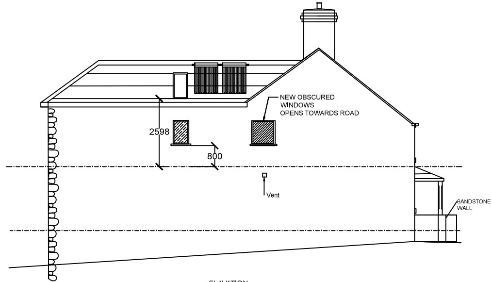
ELAVATION 2
