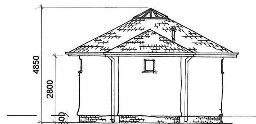
North Elevation 1 : 100
