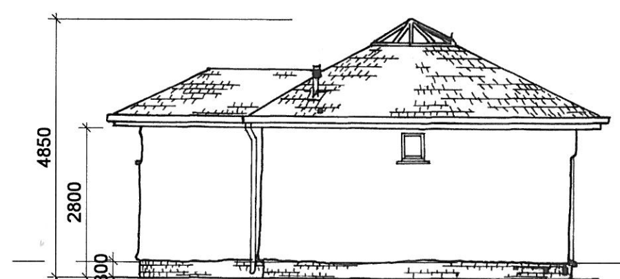
West Elevation 1 : 100
