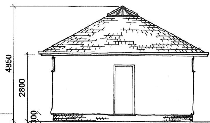
South Elevation 1 : 100
