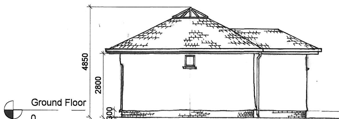
East Elevation 1 : 100
