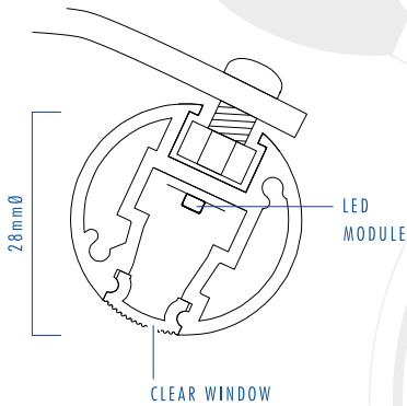
LIGHTING CANOPY SECTION THROUGH scale 1:1
