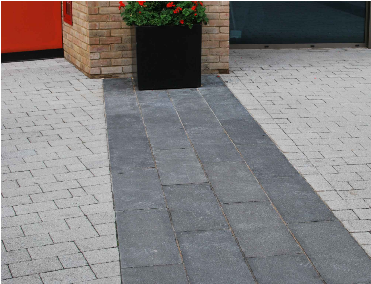
Unit paving to pedestrian circulation
