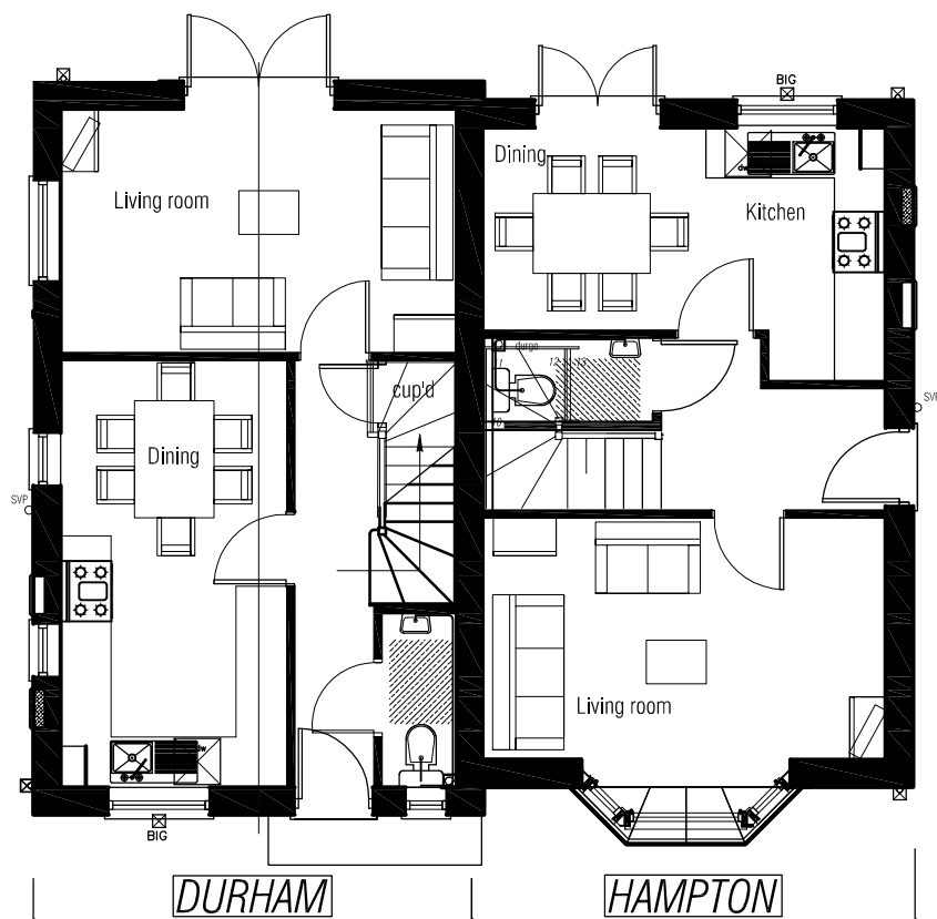
Ground Floor Layout Plan Plots 22 and 23
