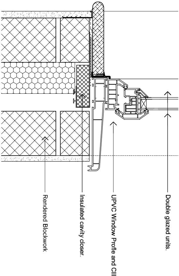
C_Cill Detail - 1:5
