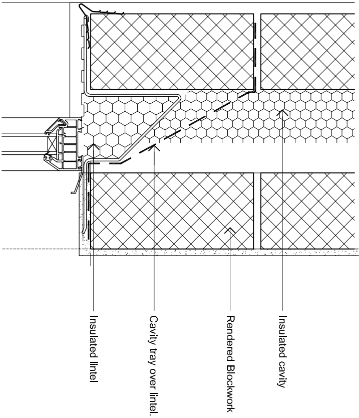
A_Head Detail - 1:5
