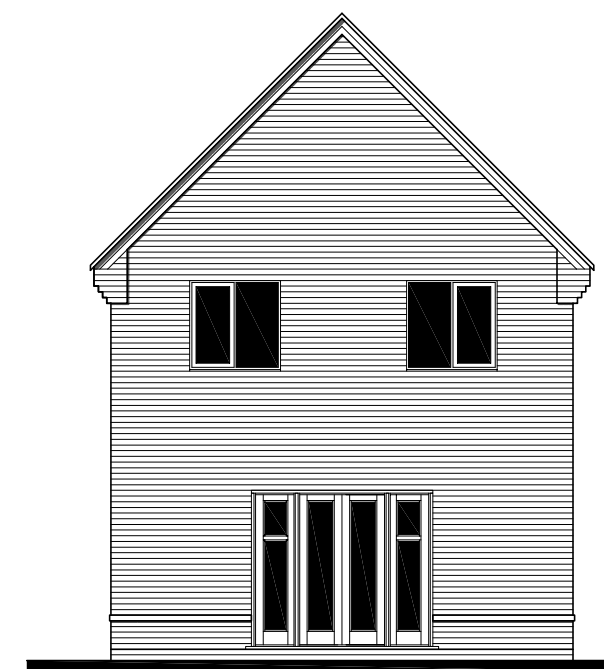
REAR ELEVATION
