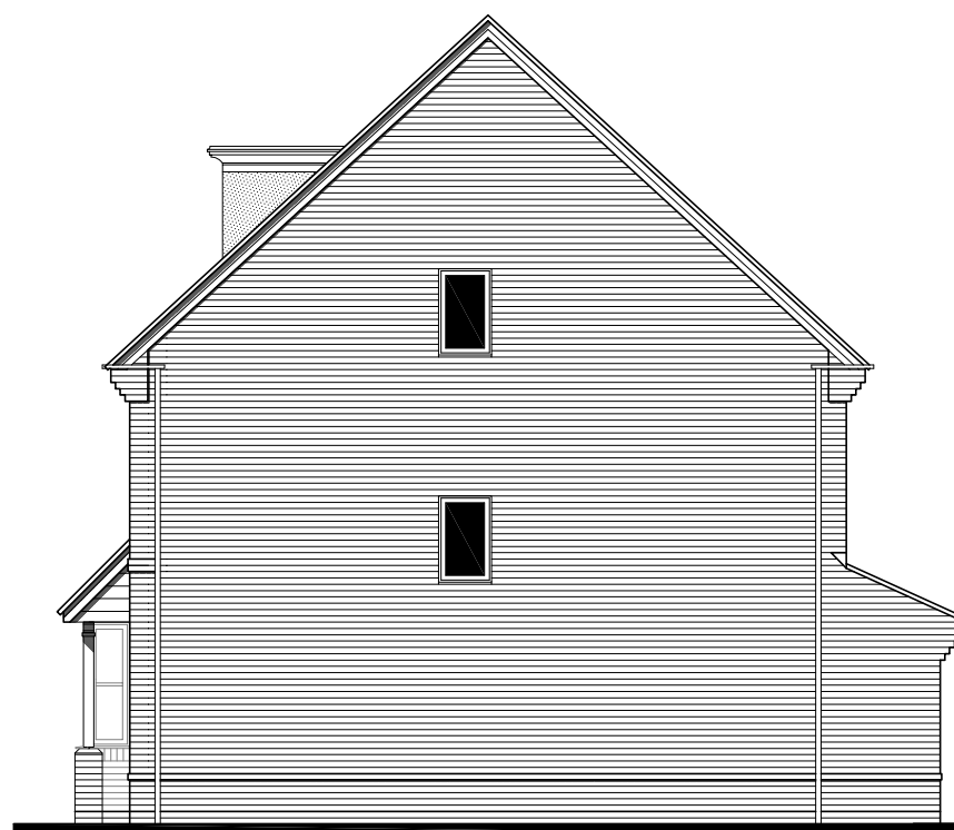
SIDE ELEVATION
