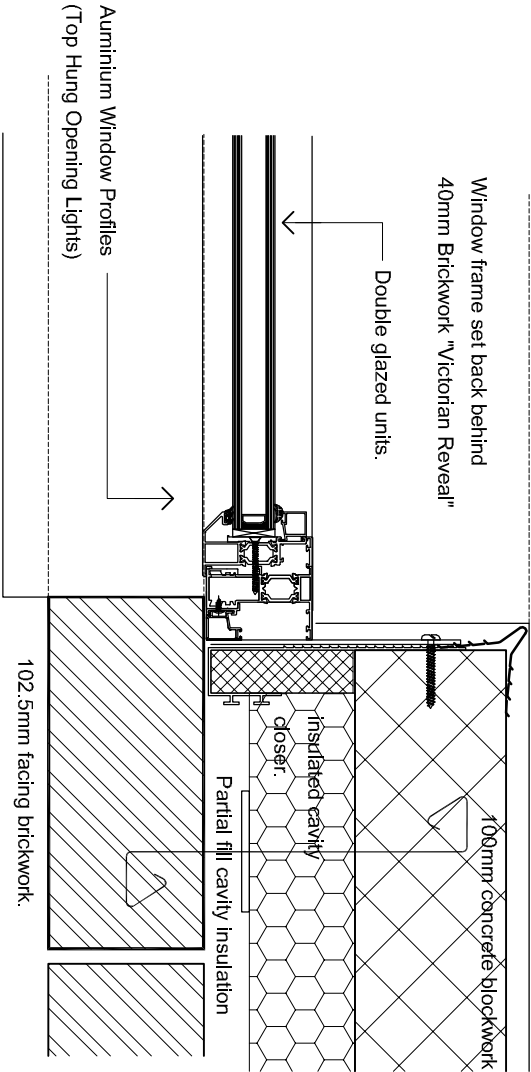
Typical Brickwork Victorian Reveal Window Jamb - 1:5
