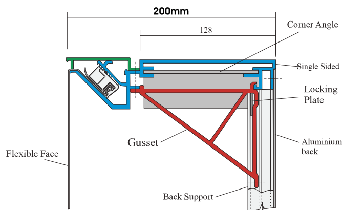
General Box Profile
