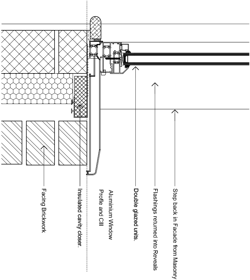
C_Cill Detail - 1:5
