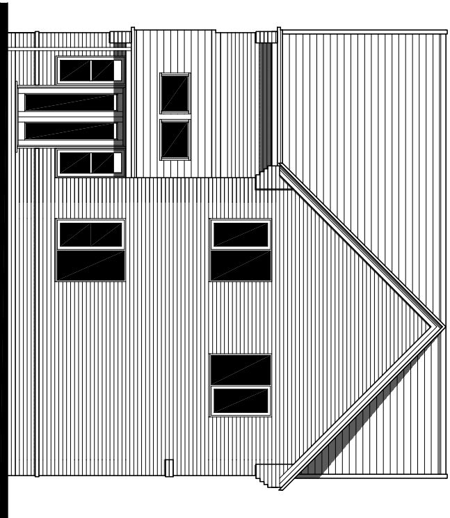
REAR ELEVATION
