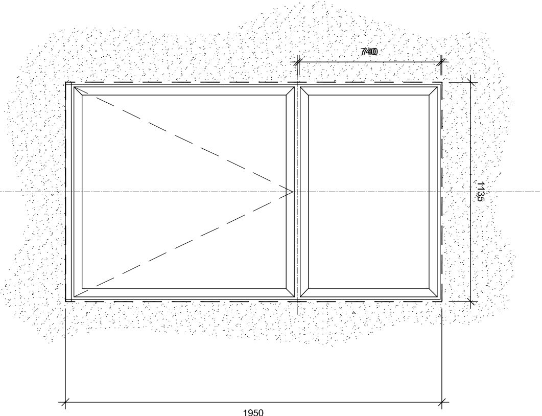
Typical Render North West Elevation - 1:20
