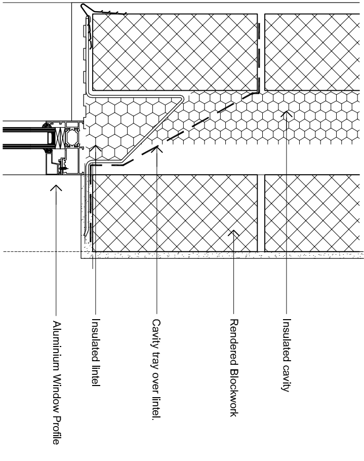
A_Head Detail - 1:5
