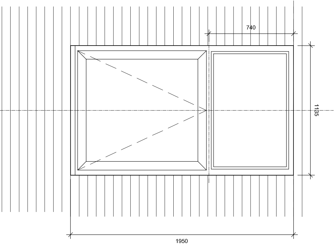
Typical Brickwork Elevation - 1:20
