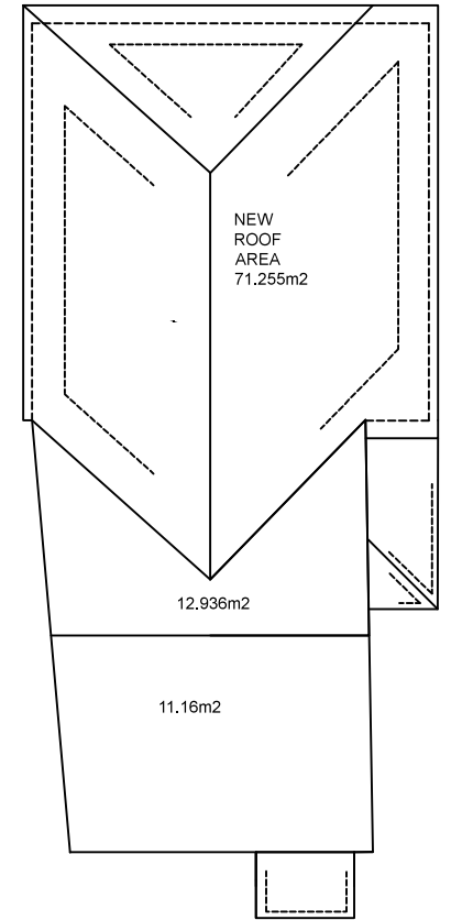
Roof Plan
