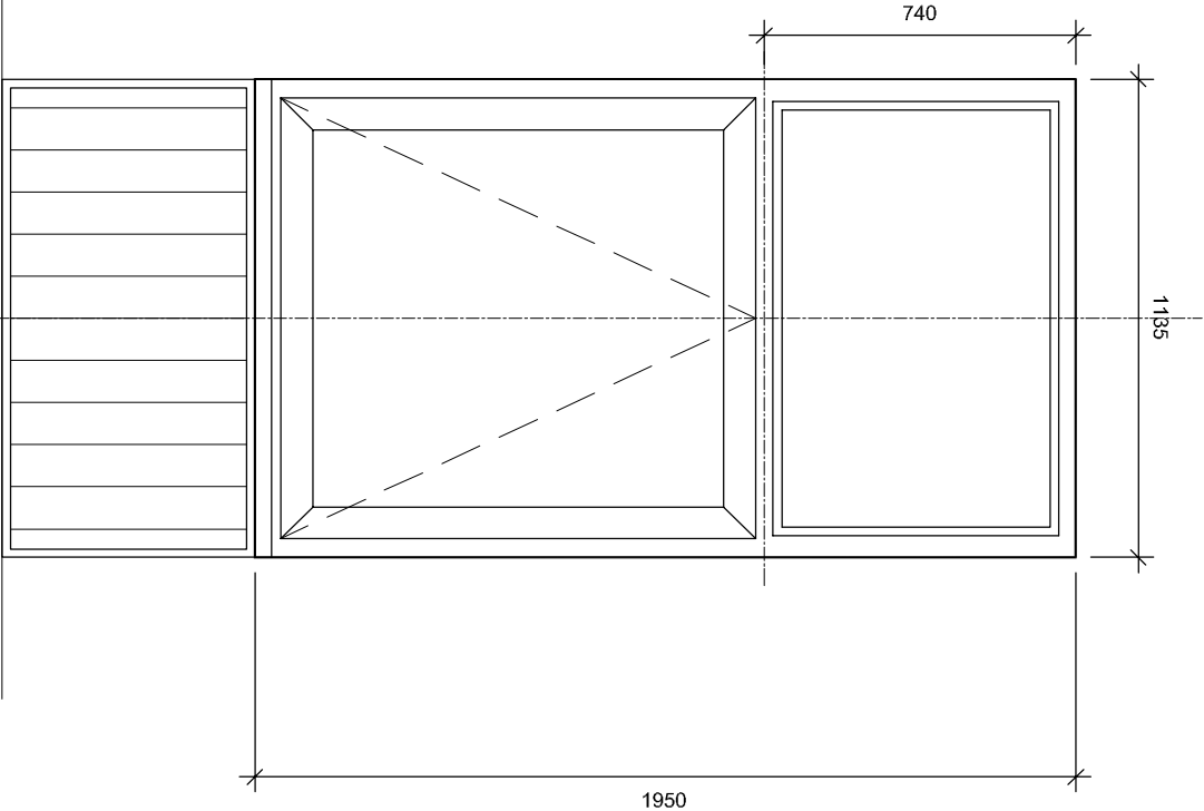
Typical Cedar Feature Elevation - 1:20
