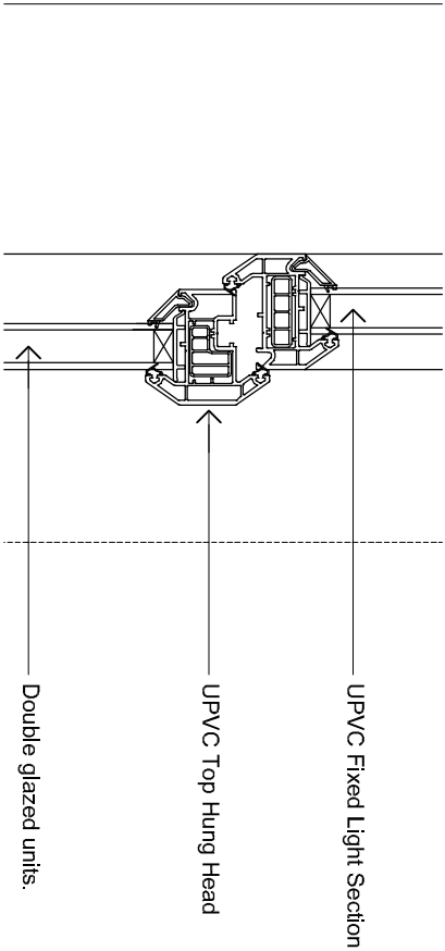
B_Transom Detail - 1:5
