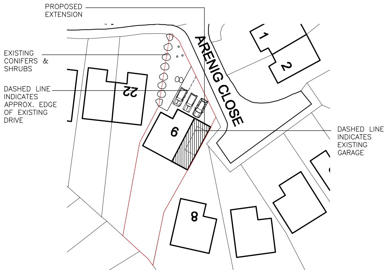
BLOCK PLAN 1:500
