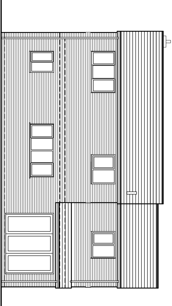
REAR ELEVATION
