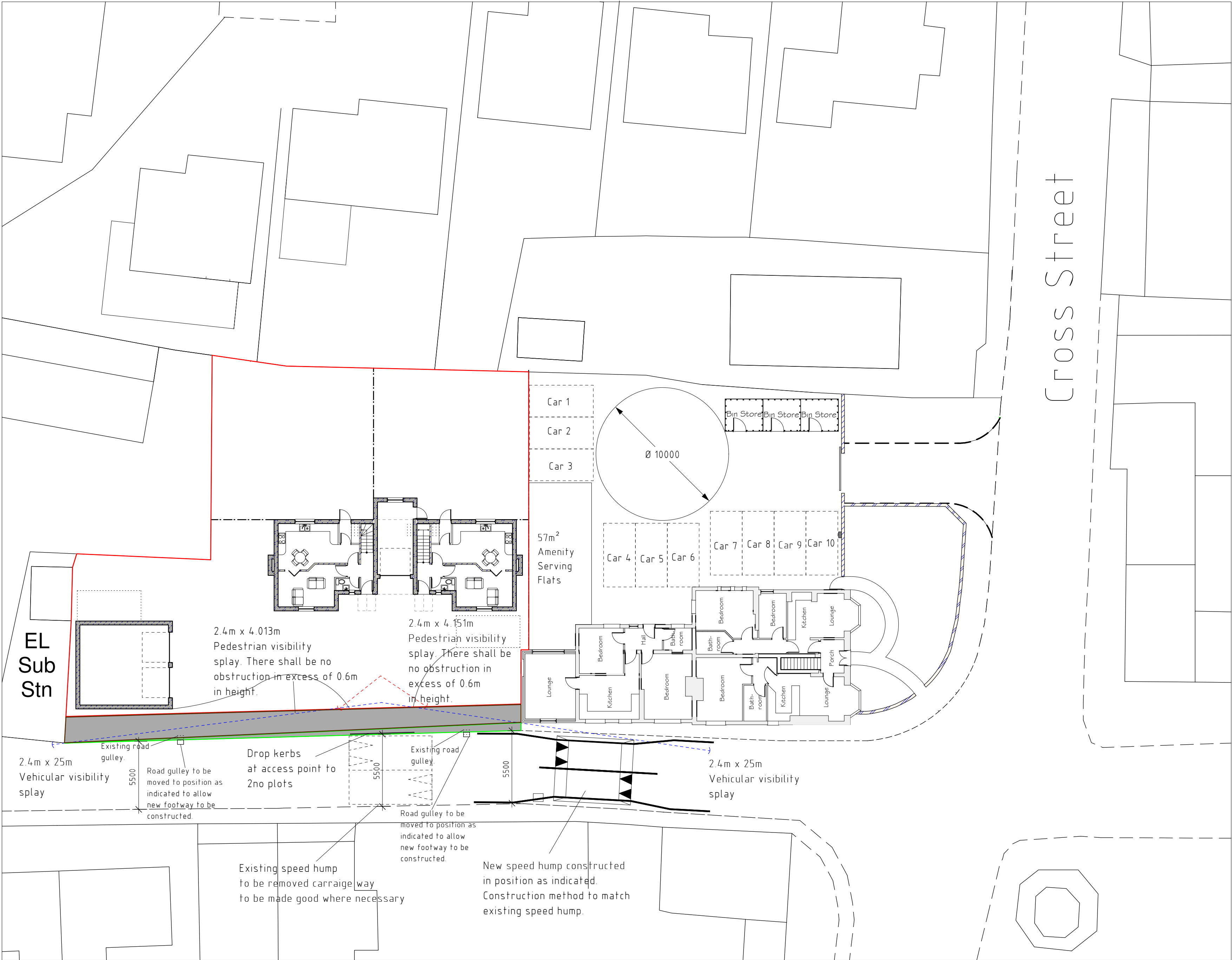
Footpath layout plan 1:200
