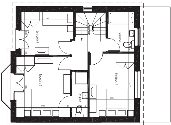
First floor plan Floor area to be created: 51m 2 / 549 sq ft
