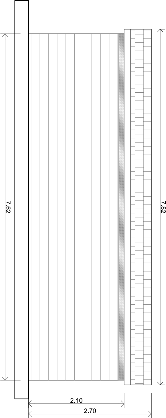
SIDE ELEVATION
