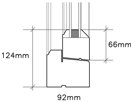
Section through sill (1:5)
