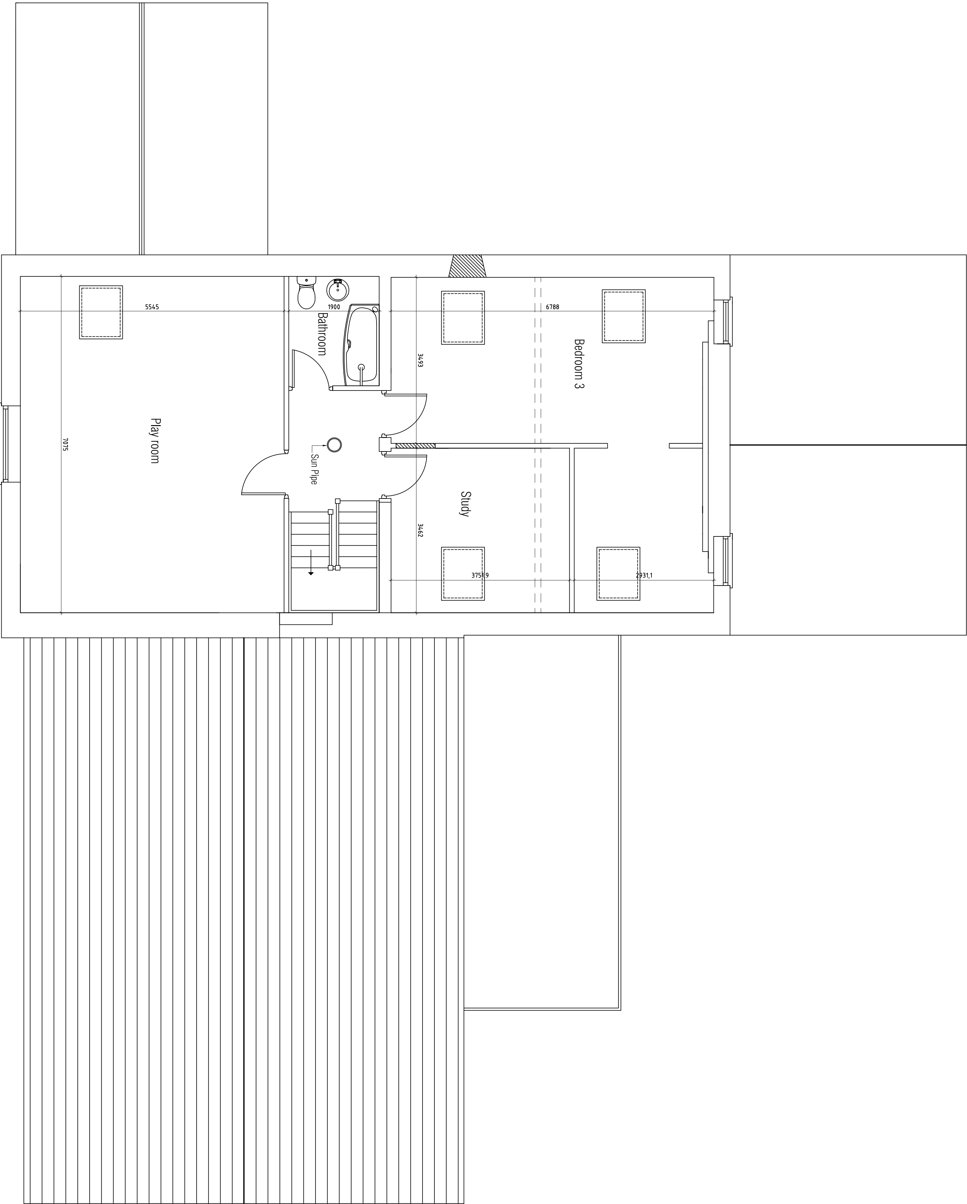
Proposed Second Floor
