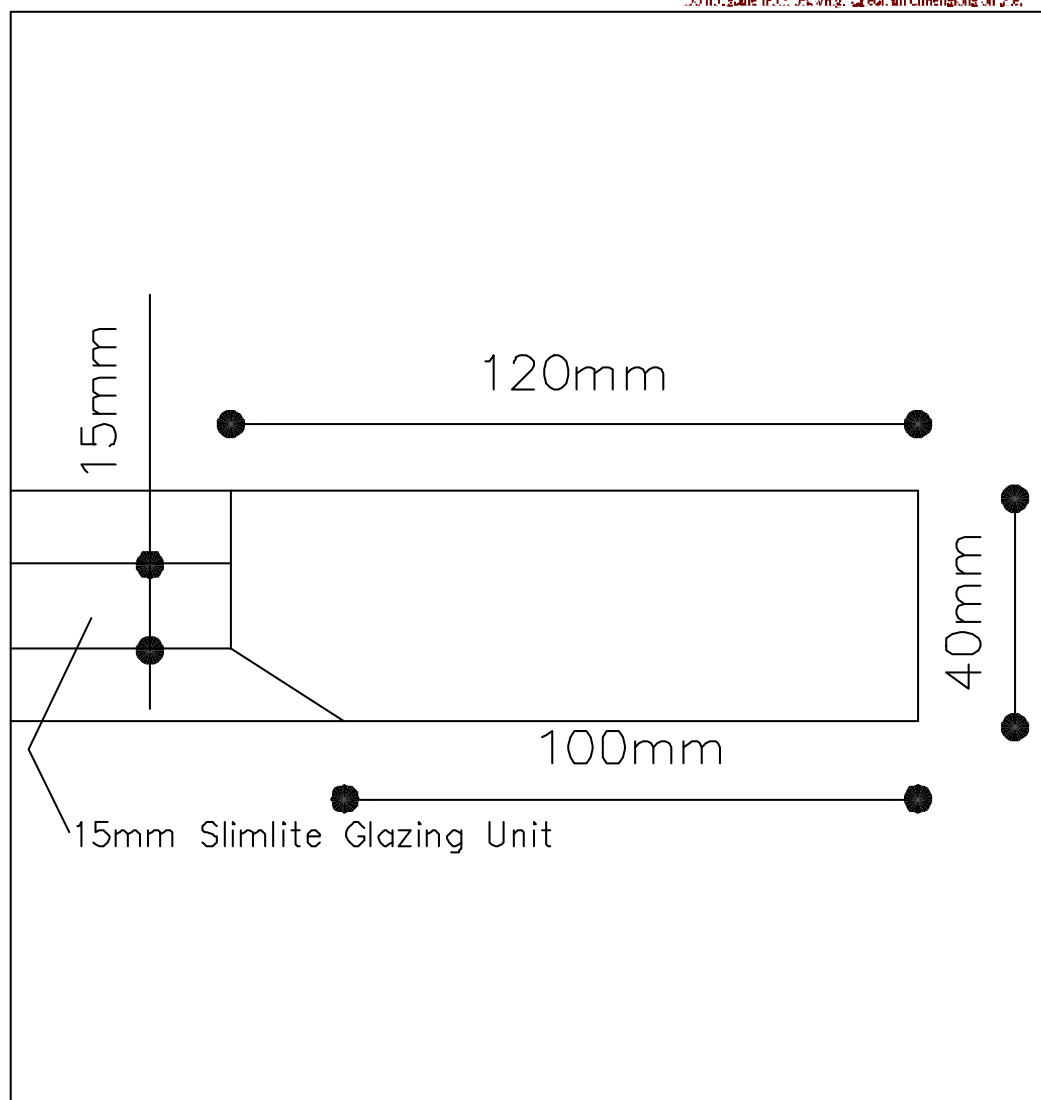
1:1 Detail of Glazed door
