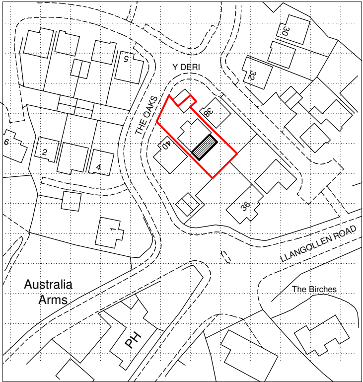
Location Plan 1:1250
