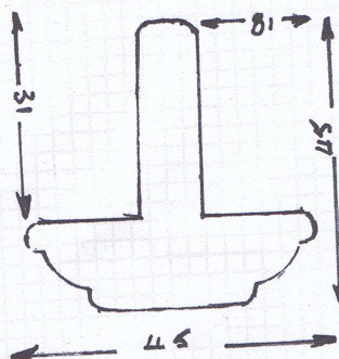
GLAZING BAR SECTION
