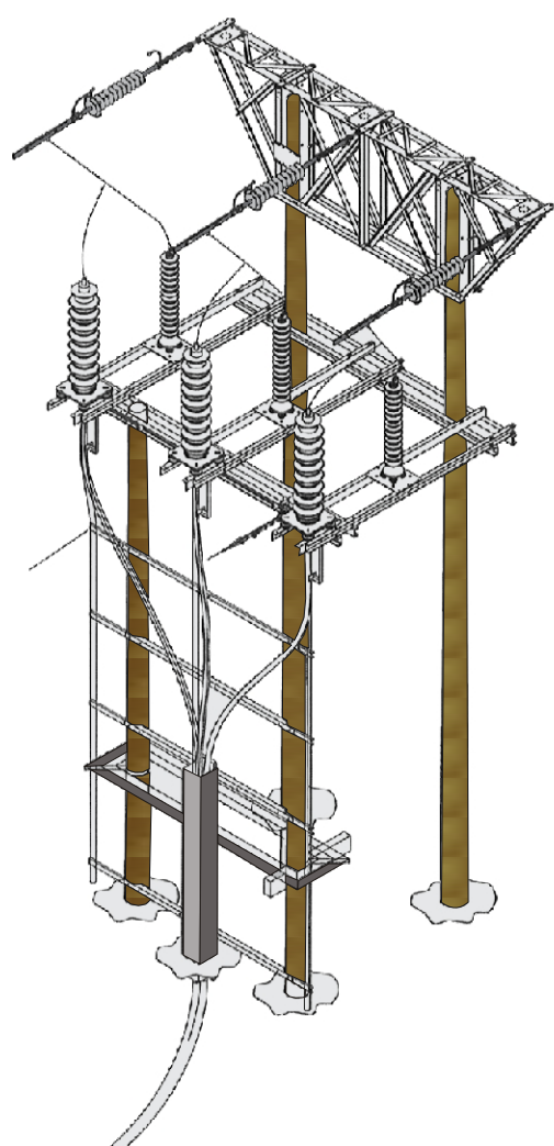
Terminal Structure
