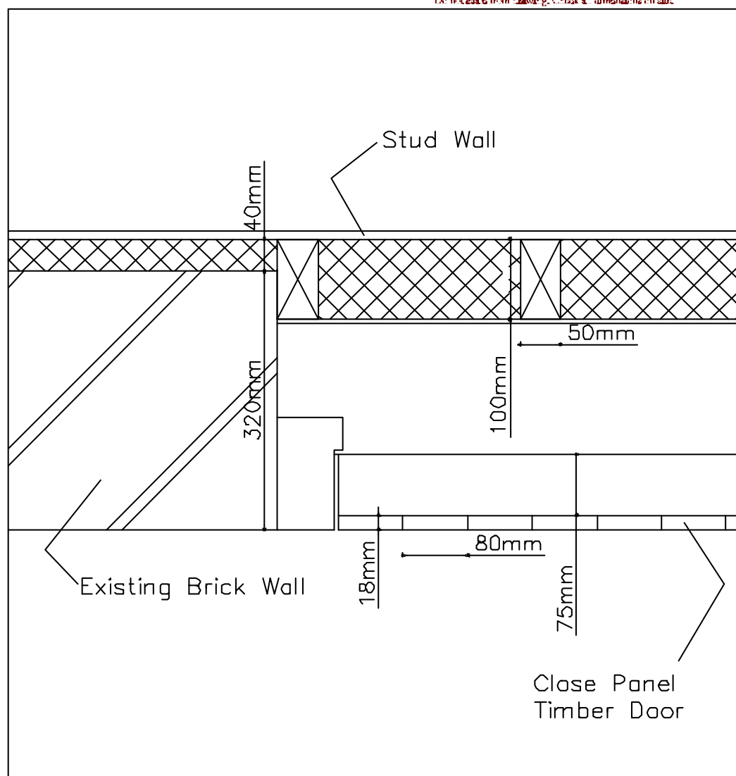
1:5 Detail of Close Panel Timber Door
