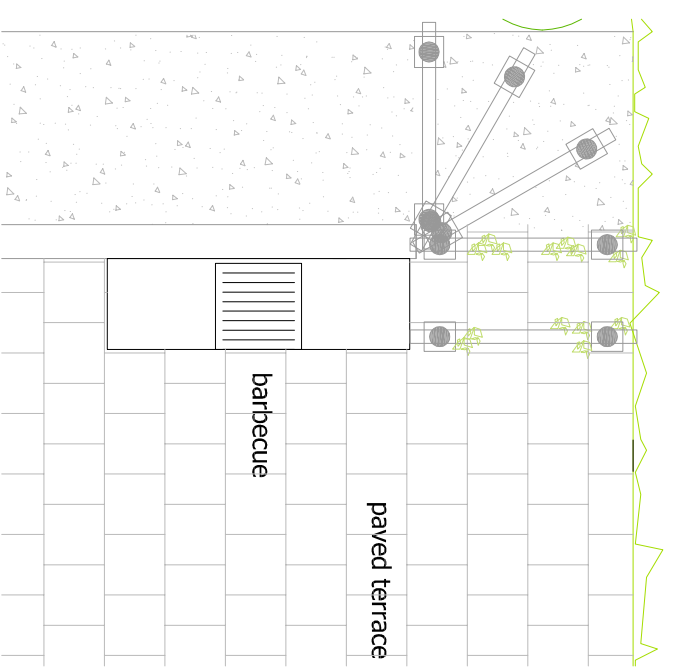
barbeque area detail @ 1:50
