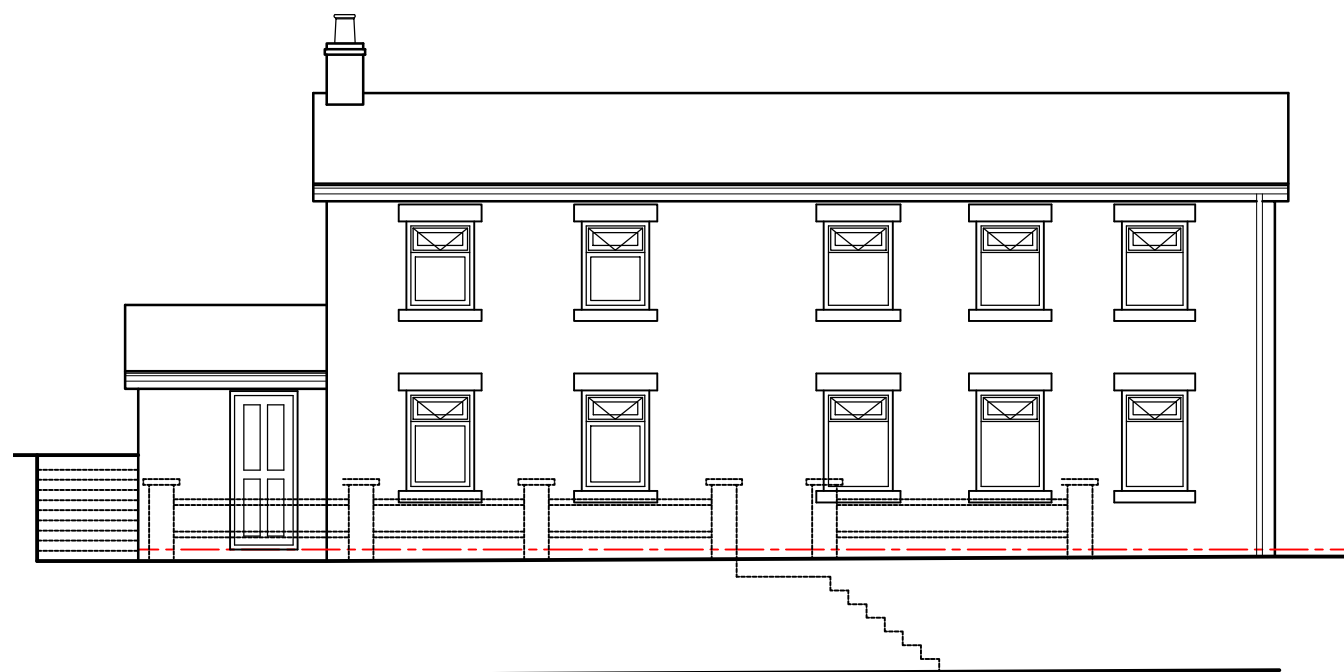
Front Elevation
