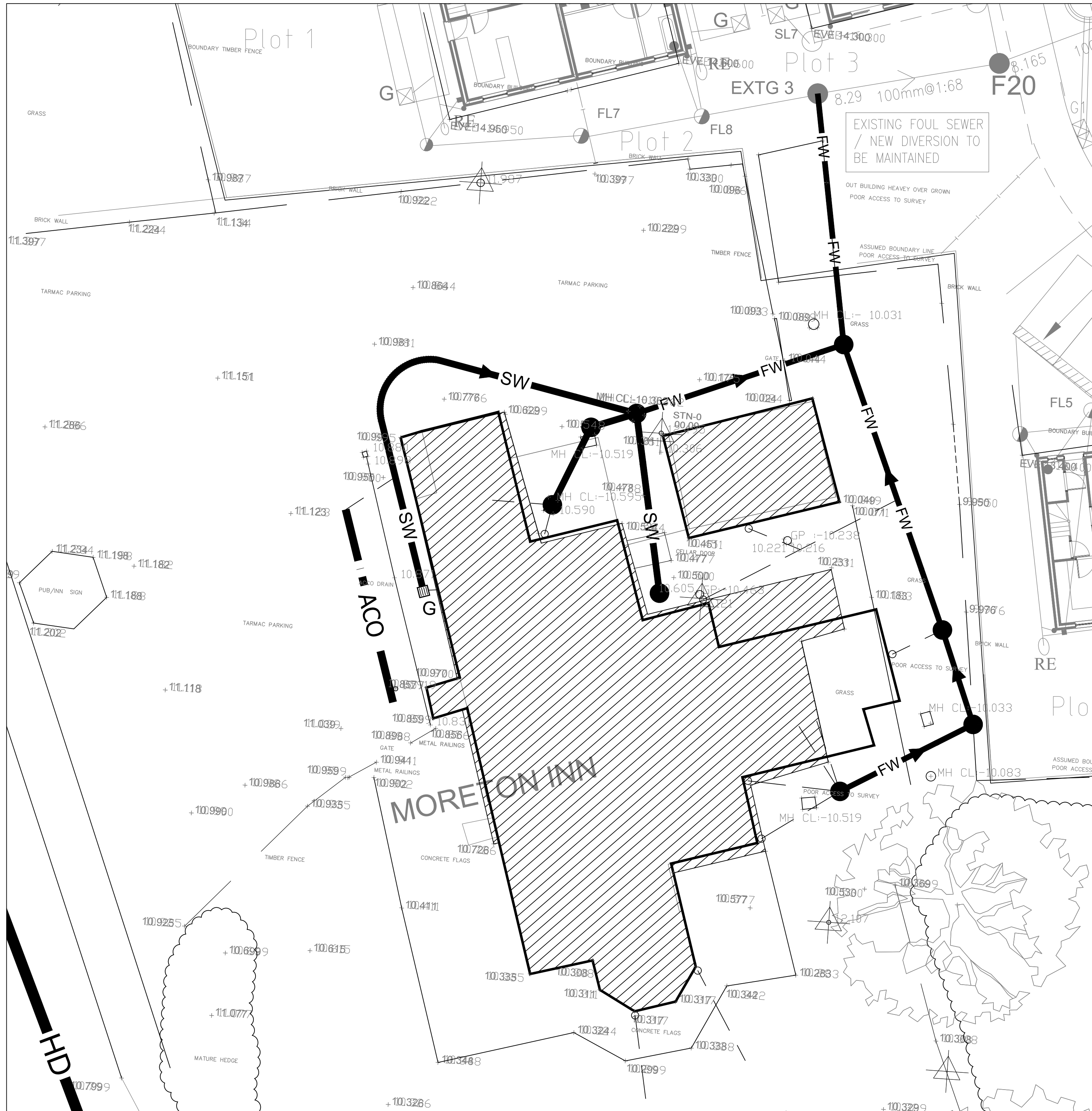
Existing Site Drainage Scale 1:125
